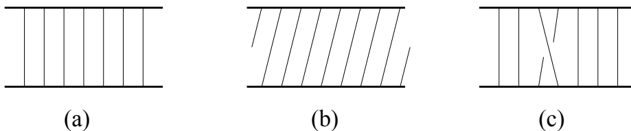
Figure 6: Possible types of contractions between fields in traces of operators, which are represented by horizontal lines. Vertical lines represent the contractions. (a) and (b) are two examples of planar contractions while (c) is an example of a non-planar contraction.
